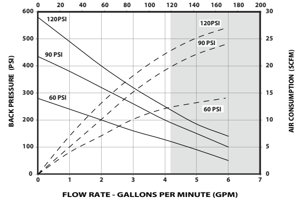
NON SHADED AREA OF THE GRAPH REPRESENTS RECOMMENDED OPERATING RANGE FOR CONTINUOUS DUTY
